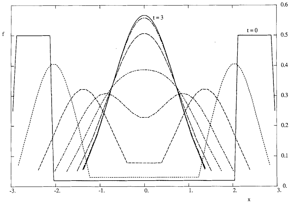
FIG. 8. Numerical solution of the model Fokker-Planck equation; 24 particles have been used. \Delta t = 0.002 . The output times are: t = 0, 0.1, 0.3, 0.5, 0.7, 1, 1.5, 3 .
