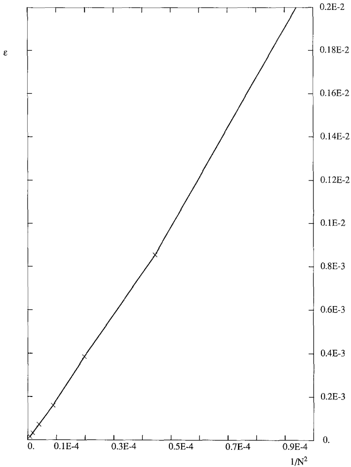
FIG. 4. Rate of convergence of the numerical scheme for the diffusion equation in unbounded domain: \varepsilon_N versus 1/N^2 .
