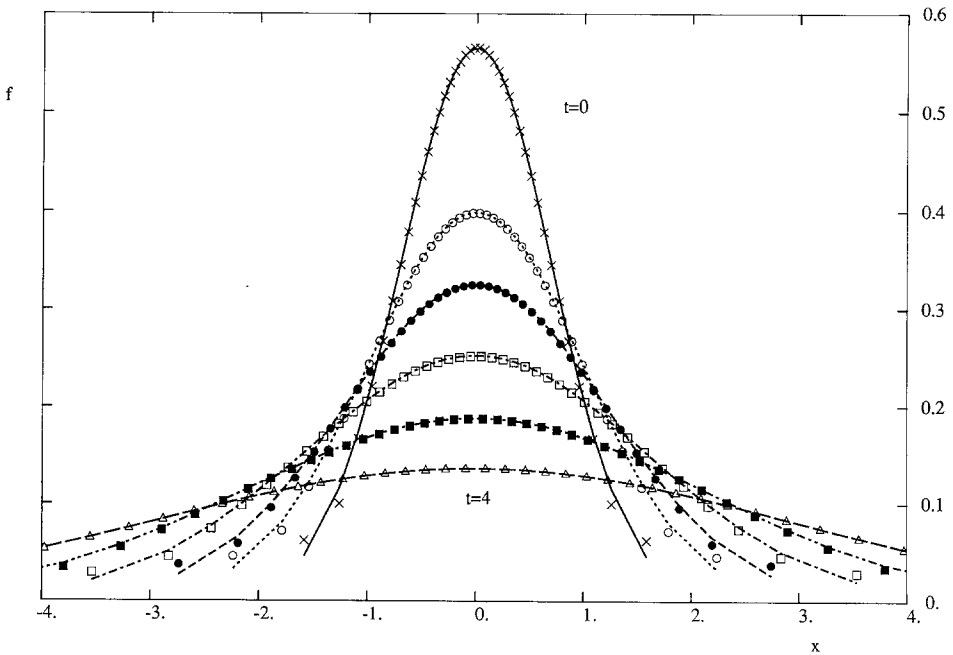
FIG. 1. Comparison between the exact (lines) and numerical (marks) solution for the diffusion equation at different times. The Forward-Euler scheme has been used with 40 particles and time step \Delta t = 0.001 . The initial profile is gaussian. The output times are: t = 0, 0.25, 0.5, 1.0, 2.0, 4.0 .
