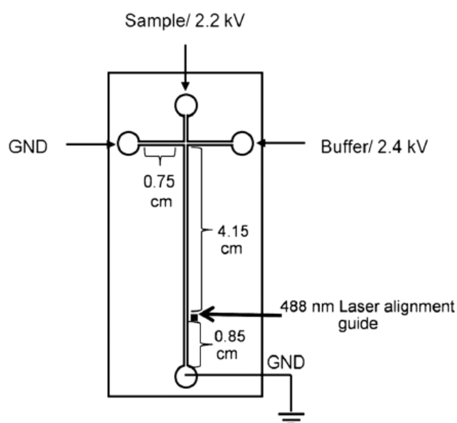
Figure 36 - A schematic of a simple “T” 5 cm microchip design with channel dimensions and applied voltages.
