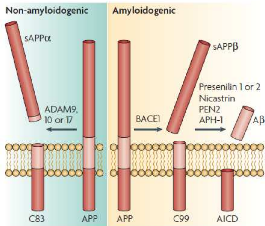
Figure 7 - APP proteolysis.
