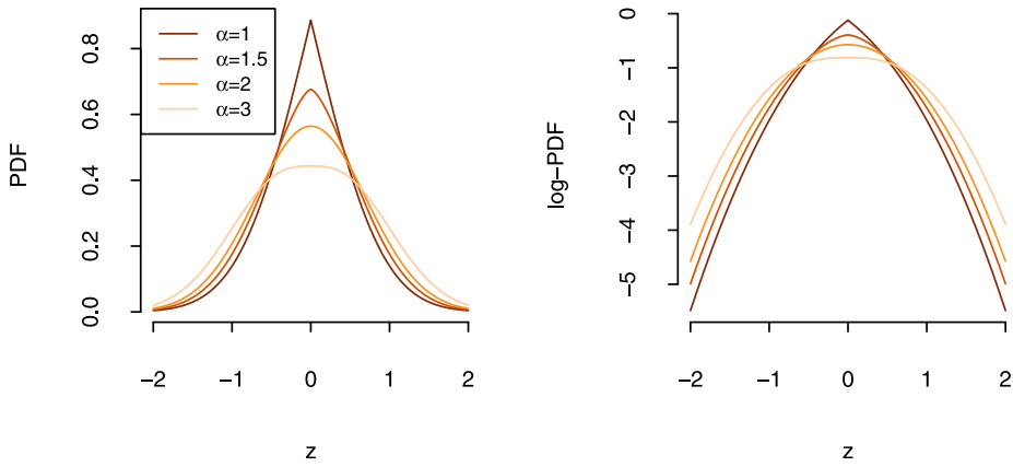
Fig. 4. Examples of BTN PDFs for different values of body shape \alpha and fixed tail shape \beta = 2 .
