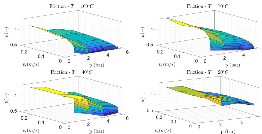
Figure 12. Dry friction coefficients on coarse granite vs. sliding velocity for different pressures and temperatures; model from [116], replotted by the authors.
