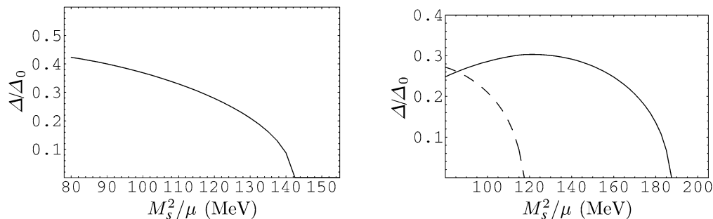
Fig. 2. Left panel: \Delta_2/\Delta_0 = \Delta_3/\Delta_0 against M_s^2/\mu , evaluated for \mu_L = 0 . Right panel: \Delta_2/\Delta_0 (dashed line) and \Delta_3/\Delta_0 (solid line) as a function of M_s^2/\mu , computed for \mu_L = 200 MeV. In both pictures T = 0.1\Delta_0 .
