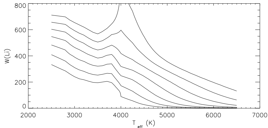
Figure 6.7: The plot shows the relation between EWs and T_{eff} at fixed Li abundance ( \log N(\text{Li}) = 0.5, 1.0, 1.5, 2.0, 2.5, 3.0, 3.5 ) and \log g = 4.5 . The final COGs is a matching and an interpolation of Palla et al. (2007) and Soderblom et al. (1993b) relations.
