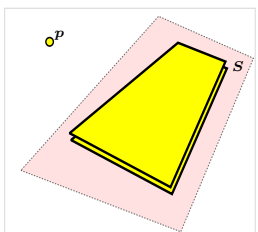
Base locus scheme \mathcal{B}(\mathcal{J}_{12}^5)
