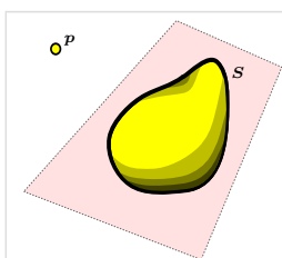
Base locus scheme \mathcal{B}(\mathcal{J}_{16}^5)
