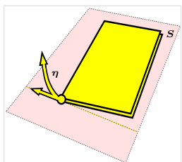
Base locus scheme \mathcal{B}(\mathcal{J}_3^5)
