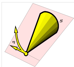
Base locus scheme \mathcal{B}(\mathcal{J}_5^5)
