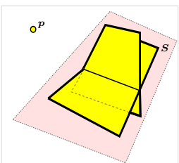
Base locus scheme \mathcal{B}(\mathcal{J}_{14}^5)
