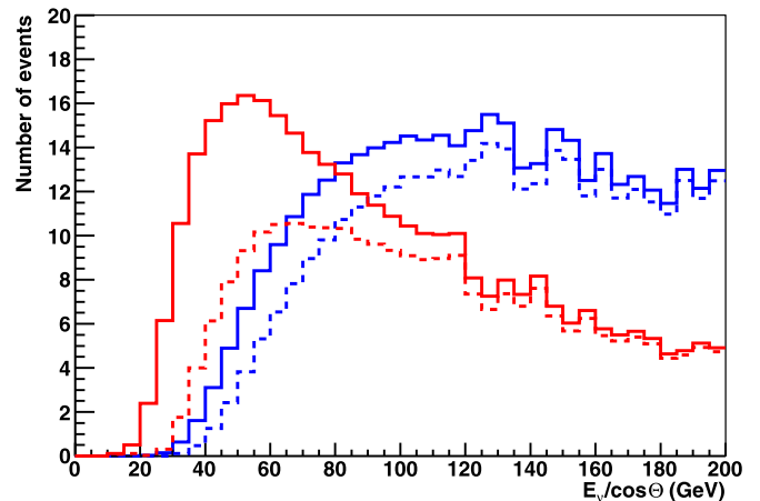
Fig. 3. Distribution of E_\nu/\cos\theta for the selected events of the atmospheric neutrino simulation. The solid lines are without neutrino oscillations, the dashed lines include oscillations assuming the best fit values reported in [3]. The red histograms indicate the contribution of the single-line sample, in blue the multi-line events. (For interpretation of the references to colour in this figure legend, the reader is referred to the web version of this Letter.)
