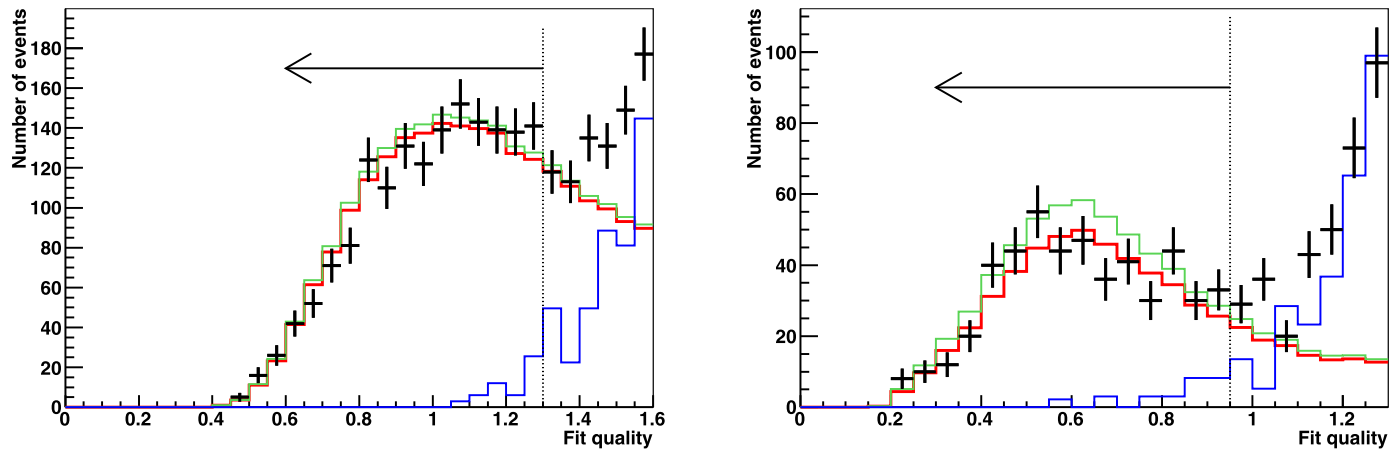
Fig. 2. Normalised fit quality of the final multi-line (left) and single-line (right) samples. Data with statistical errors (black) are compared to simulations from atmospheric neutrinos with oscillations assuming parameters from [3] (red) and without oscillations (green) and atmospheric muons (blue). For a fit quality larger than 1.6 (multi-line) or 1.3 (single-line) the misreconstructed atmospheric muons dominate. The arrows indicate the chosen regions. (For interpretation of the references to colour in this figure legend, the reader is referred to the web version of this Letter.)
