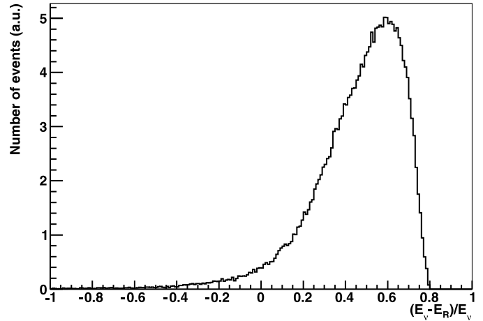
Fig. 1. Difference between the true neutrino energy, E_\nu , and E_R normalised by E_\nu for low energy events ( E_\nu < 100 GeV) from the final event sample of Section 6.
