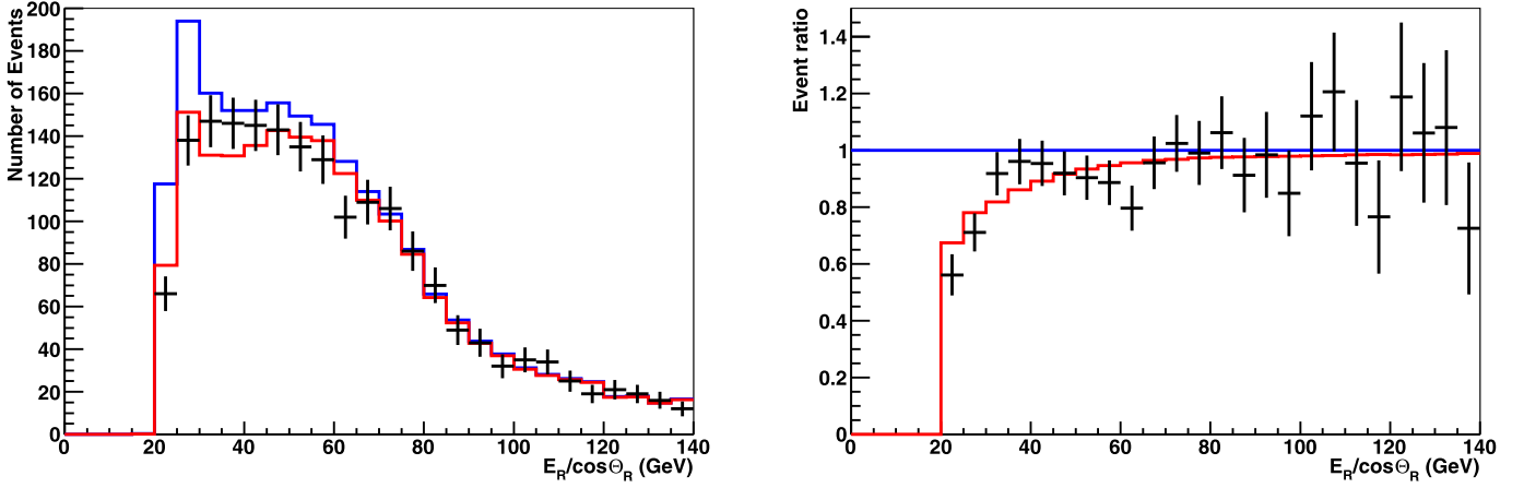
Fig. 4. Left: Distribution of E_R/\cos\theta_R for selected events. Black crosses are data with statistical uncertainties, whereas the blue histogram shows simulations of atmospheric neutrinos without neutrino oscillations (scaled down by a factor 0.86) plus the residual background from atmospheric muons. The red histogram shows the result of the fit. Right: The fraction of events with respect to the non-oscillation hypothesis. Same colour code as for the left figure. (For interpretation of the references to colour, the reader is referred to the web version of this Letter.)
