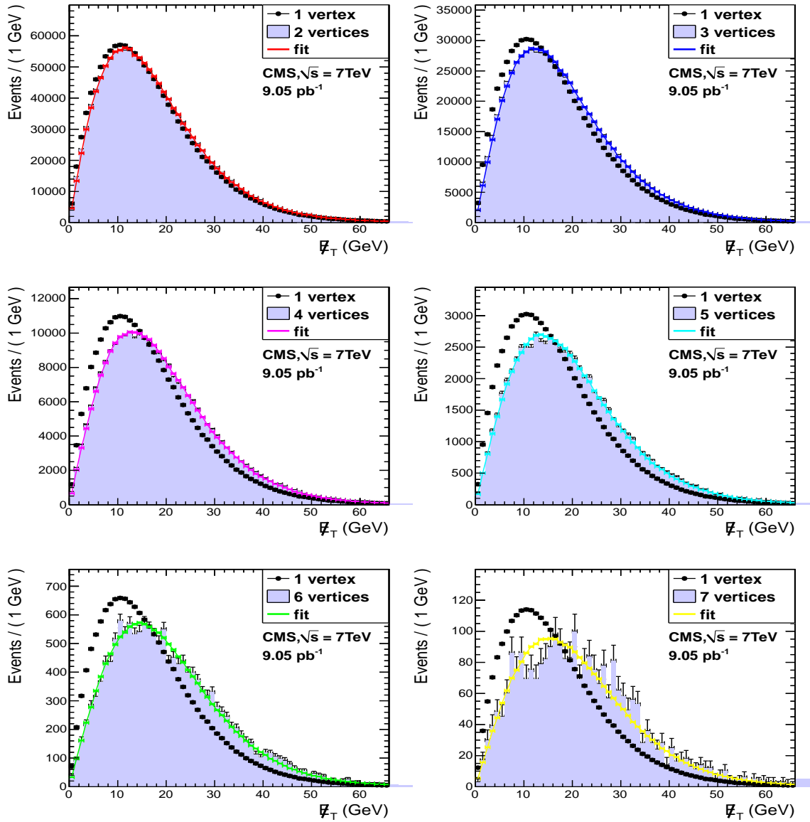
Figure 18. PF E_T distributions in pile-up events. The figures show a comparison between the one- and n -vertex shapes ( n = 2, \dots, 7 ) and the results of a simultaneous fit of eq. (6.2) to the n -vertex shapes. The one-vertex distribution is normalized to the n -vertex distribution for each plot.
