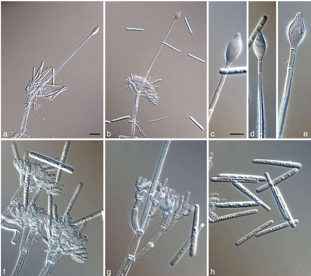
Fig. 3 Calonectria pseudomexicana . a, b. Macroconidiophores; c–e. fusiform to broadly ellipsoidal vesicles with papillate apices; f, g. conidiogenous apparatus with conidiophore branches and doliform to reniform phialides; h. 1-septate macroconidia. — Scale bars = 10 \mu m.
