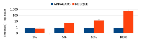
Fig. 4. Running times of APPAGATO and RESQUE on the functional interaction networks. Results are grouped by the similarity thresholds. The running time of RESQUE highly depends on the number of target nodes that can be matched with a query node (i.e., on the similarity threshold t ).
