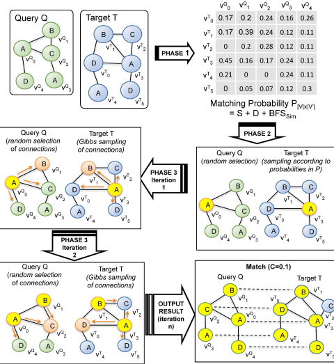
Fig. 1. The APPAGATO approximate matching algorithm.
