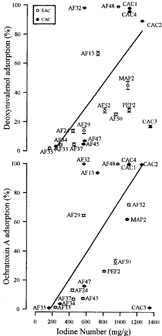
FIGURE 3. Relationship between iodine number and the ability to adsorb ochratoxin A (4 \mu g/ml) and deoxynivalenol (4 \mu g/ml) from 5 ml of aqueous solution by 2 mg (for ochratoxin A) and 10 mg (for deoxynivalenol) of the following sorbents: experimental activated carbons (EAC) obtained from olive residues (AF), peach stones (PEP), and almond shells (MAP), and commercial activated carbons (CAC). Each point represents the mean, n = 3 ; error bars denote standard error of the mean. Values of the linear equations are: ochratoxin A adsorption = 0.09 iodine number - 15.98 ( r^2 = 0.56 ). Deoxynivalenol adsorption = 0.08 iodine number - 16.67 ( r^2 = 0.47 ). CAC3 was not considered a data point of the regressions.
