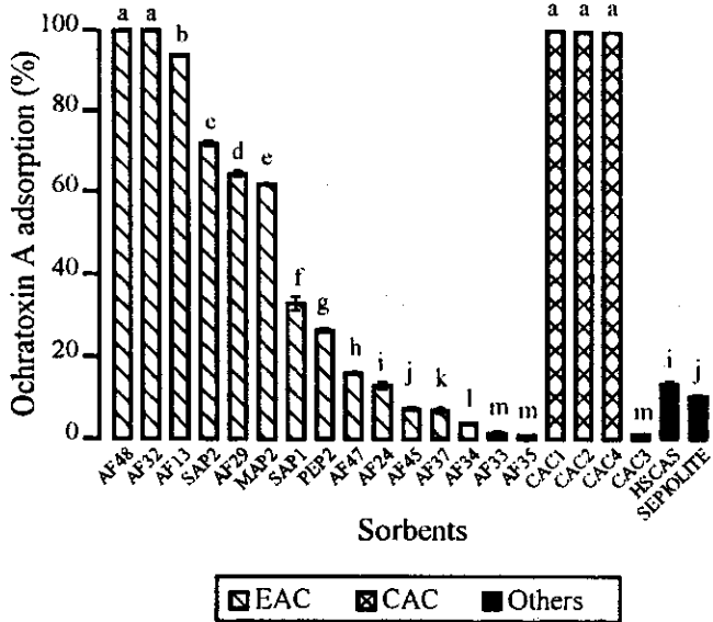
FIGURE 1. Adsorption of ochratoxin A (4 \mu\text{g}/\text{ml} ) and deoxynivalenol (4 \mu\text{g}/\text{ml} ) from aqueous solution by 2 mg (for ochratoxin A) and 10 mg (for deoxynivalenol) of the following sorbents: experimental activated carbons (EAC) obtained from olive residues (AF), peach stones (PEP), and almond shells (MAP); commercial activated carbons (CAC), hydrated sodium calcium aluminosilicate (HSCAS) and sepiolite (S). Each bar represents the mean, n = 3 ; error bars denote standard error of the mean; different letters on bar tops mean significantly different ( P < 0.05 ).
