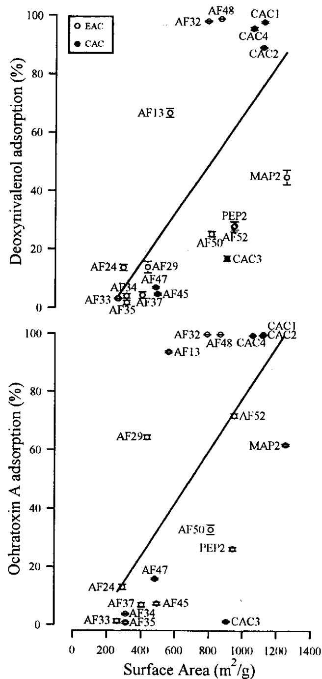
FIGURE 2. Relationship between the surface area and the ability to adsorb ochratoxin A (4 \mu g/ml) and deoxynivalenol (4 \mu g/ml) from aqueous solution by 2 mg (for ochratoxin A) and 10 mg (for deoxynivalenol) of the following sorbents: experimental activated carbons (EAC) obtained from olive residues (AF), peach stones (PEP), and almond shells (MAP), and commercial activated carbons (CAC). Each point represents the mean, n = 3 ; error bars denote standard error of the mean. Values of the linear equations are: ochratoxin A adsorption = 0.09 surface area - 12.05 ( r^2 = 0.58 ); deoxynivalenol adsorption = 0.08 surface area - 17.95 ( r^2 = 0.51 ). CAC3 was not considered as a data point of the regressions.
