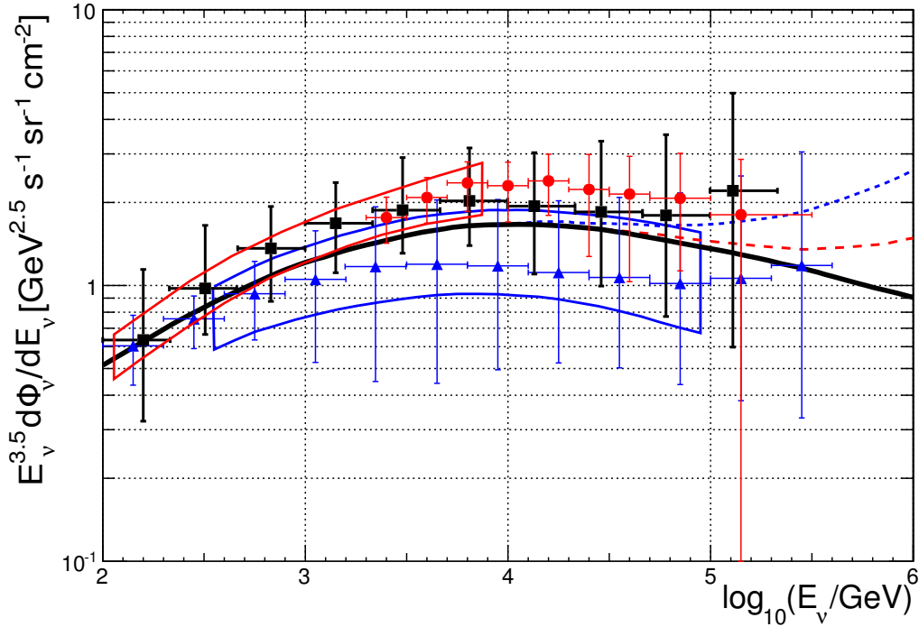
Figure 7: The atmospheric neutrino energy spectrum E_\nu^{3.5} d\Phi_\nu/dE_\nu measured in this work in the zenith angle region \theta > 90^\circ (black full squares). The full line represents the \nu_\mu flux from Ref. [20]. The red and blue dashed lines include two prompt neutrino production models from Ref. [24] and Ref. [25], respectively. All theoretical expectations are zenith-averaged from 90^\circ to 180^\circ . The result of the AMANDA-II unfolding [12] averaged in the region 100^\circ to 180^\circ is shown with red circles and that of IceCube40 [13] zenith-averaged from 97^\circ to 180^\circ is shown with blue triangles. The red region corresponds to the \nu_\mu measurement from Ref. [11], and the blue one the IC40 update from Ref. [49].
