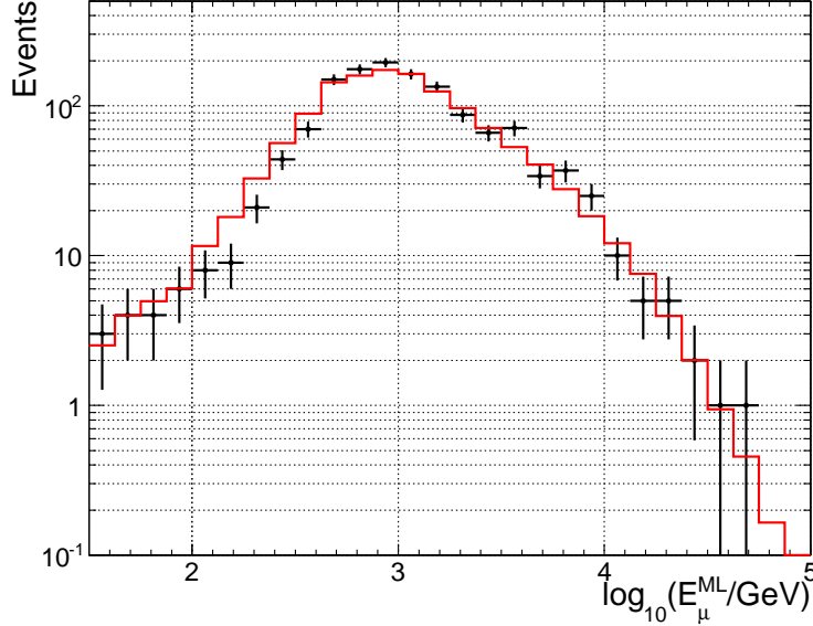
Figure 3: Data (black crosses) and Monte Carlo (red line) comparison for the maximum likelihood muon energy estimator E_{\mu}^{ML} , for events passing the selection cuts. This distribution is obtained at the end of the procedure, after the data unblinding (see text). The Monte Carlo prediction is scaled by a factor 1.25.
