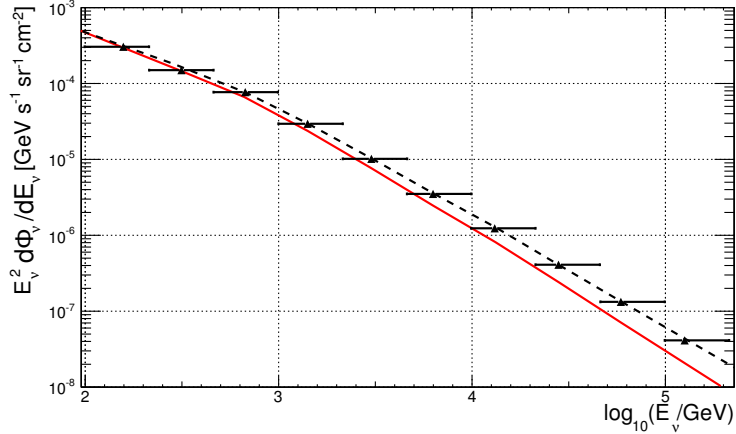
Figure 2: Unfolding of a known spectrum. The red solid line is the energy spectrum from Ref. [20] used as the a priori probability for the bayesian unfolding of pseudo-data generated according to an injected spectrum (black dashed line). The unfolding result (black symbols) is shown without error bars.
