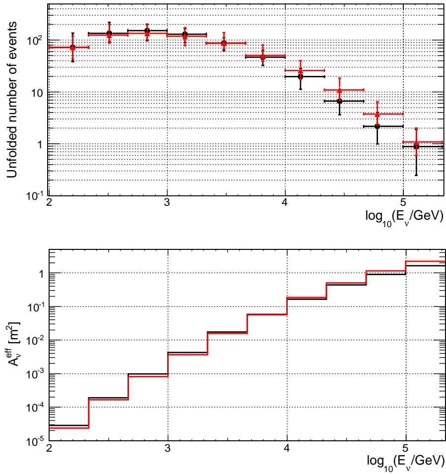
Figure 4: Top: unfolded energy distribution at the detector for the energy likelihood (red) and the energy loss (black) methods. The numbers correspond to events per bin per year of effective livetime. Bottom: corresponding neutrino effective area for upgoing neutrinos for the two methods.
