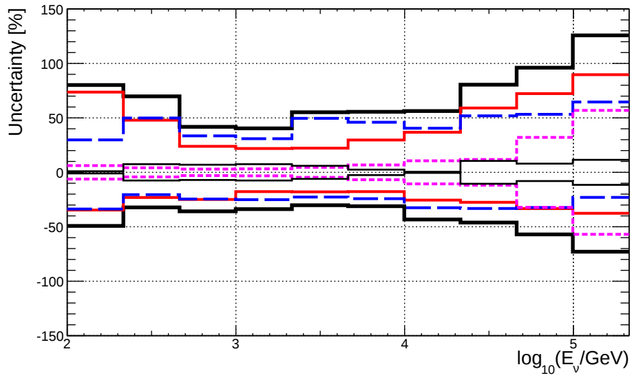
Figure 6: Systematic uncertainties calculated for each neutrino energy bin. Red continuous line represents the effects given by a \pm 10\% change of the OM efficiency with respect to the default value; blue dashed line is for a \pm 10\% change in the absorption length in water; magenta short dashed line is the statistical uncertainties. The thick black line shows the estimated total uncertainty while the thin black line represents the relative difference between the two unfolding results. The effects from the OM angular acceptance and the change in the underlying event weighting model (see text) are not shown in the figure.
