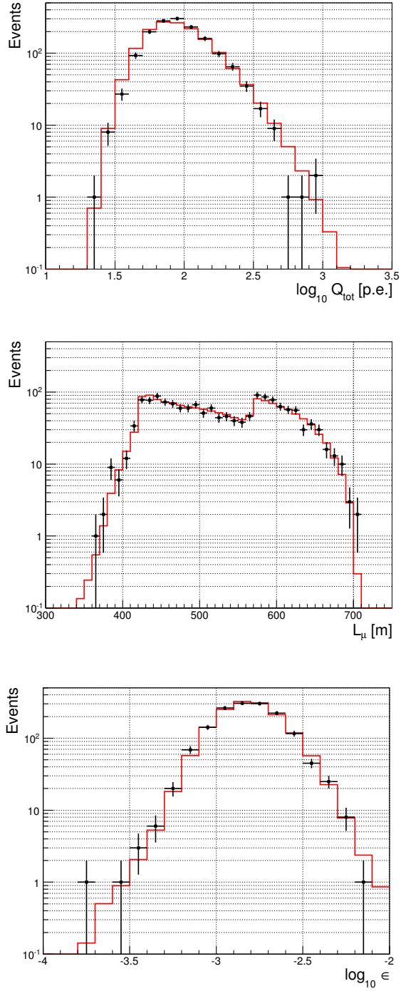
Figure 1: Comparison between data (black crosses) and simulations (red line) for the quantities used to construct the energy loss estimator \rho , Eq. 7. (Top) Distribution of the total measured amplitude Q_{tot} (in photoelectrons) on the optical modules involved in the events; (Middle) muon track length in the detector region; (Bottom) light collection capability defined in Eq. 8. Only events passing the selection criteria of the energy loss method are drawn. The Monte Carlo prediction is scaled by a factor 1.25.
