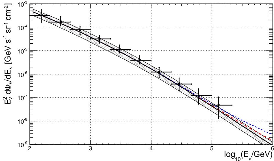
Figure 5: Atmospheric neutrino energy spectrum obtained with the ANTARES neutrino telescope using 2008-2011 data. The flux reported here is multiplied by E^2 and compared with the expectations from Ref. [20]. The gray band corresponds to the uncertainty in the flux calculation from Ref. [22]. The flux obtained by adding to the conventional flux the prompt contributions from Ref. [24] (red - dashed line) and Ref. [25] (blue - short dashed line) is also drawn.
