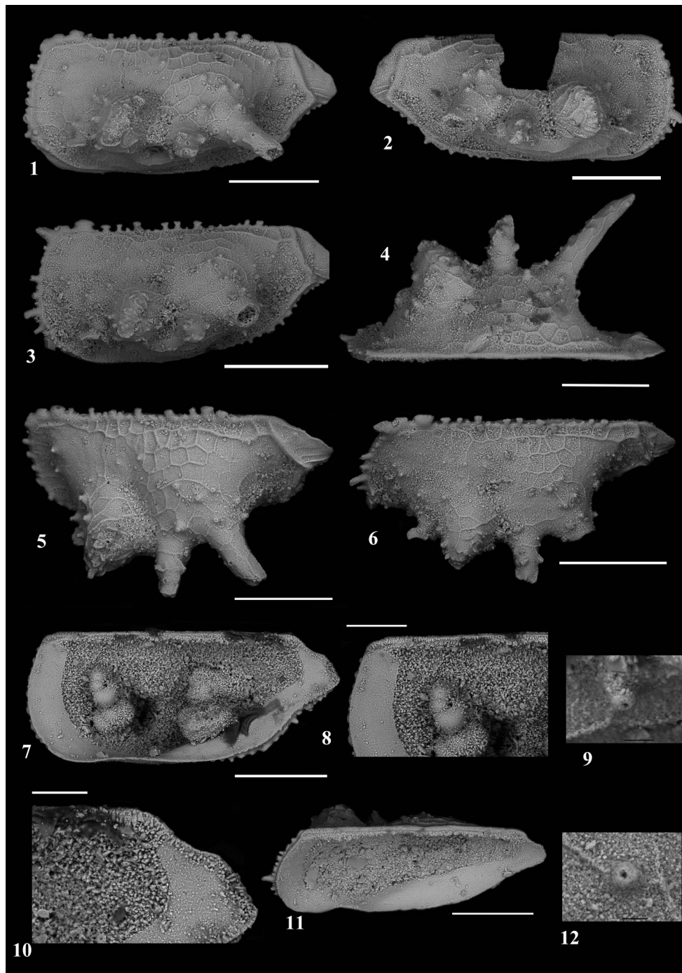
FIGURE 4. Nemoceratina (Pariceratina) barrieri n. sp. 4.1 , Left valve, Paratype PMC. O 30P 30/7/2013, external lateral view (scale bar 200 \mu\text{m} ). 4.2 , Right valve, Paratype PMC. O 31P 30/7/2013, external lateral view (scale bar 200 \mu\text{m} ). 4.3 , Left valve, Paratype PMC. O 32P 30/7/2013, external lateral view (scale bar 200 \mu\text{m} ). 4.4 , Right valve, Holotype PMC. O 9H 30/7/2013, external dorsal view (scale bar 200 \mu\text{m} ). 4.5 , Left valves, Paratypes PMC. O 30P 30/7/2013, external dorsal view partially slanting (scale bar 200 \mu\text{m} ). 4.6 , Left valves, Paratypes PMC. O 32P 30/7/2013, external dorsal view partially slanting (scale bar 200 \mu\text{m} ). 4.7 , Right valve, Paratype PMC. O 33P 30/7/2013, internal lateral view (scale bar 200 \mu\text{m} ). 4.8 , Right valve, Paratype Paratype PMC. O 33P 30/7/2013, internal lateral view, detail of the anterior marginal area (scale bar 100 \mu\text{m} ). 4.9 , External lateral view, Paratypes PMC. O 32P 30/7/2013, normal pores (scale bar 10 \mu\text{m} ). 4.10 , Right valve, Paratype Paratype PMC. O 33P 30/7/2013, internal lateral view, detail of the posterior marginal area (scale bar 50 \mu\text{m} ). 4.11 , Right valve, Paratype PMC. O 34P 30/7/2013, internal lateral view, partially slanting (scale bar 200 \mu\text{m} ). 4.12 , External lateral view, Paratypes PMC. O 32P 30/7/2013, normal pores (scale bar 10 \mu\text{m} ).
