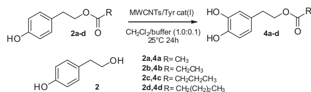
Scheme 2. Oxidation of compounds 2a–d with MWCNT/Tyr.
