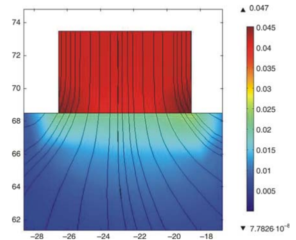
Figure 8. Simulation 2 bis – Inlet without circular joints
