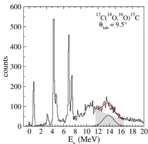
Figure 2. Energy spectra for the ^{13}\text{C}(^{18}\text{O}, ^{16}\text{O})^{15}\text{C} reaction. The linear background model, the fit of the GPV bump and their sum are shown as the grey area, the black Gaussian and the red line, respectively.
