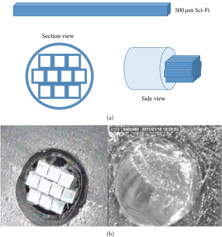
FIGURE 3: (a) The optical coupling scheme and (b) photographs of the Sci-Fi and clear fiber prepared for coupling.
