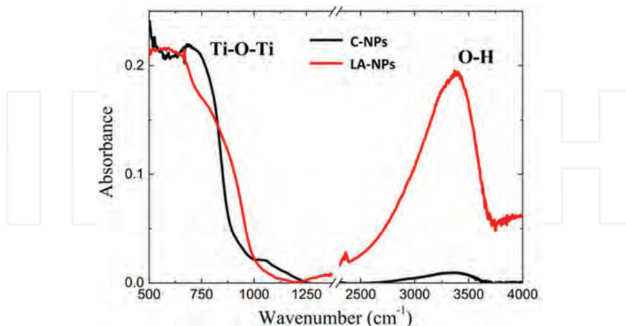
Figure 21. FTIR spectra of crystalline TiO 2 (C-NPs), and laser ablated nanoparticles (LA-NPs). Ti–O–Ti vibration and O–H stretching bands are referred in the Figure. Reprinted with permission from Zimbone et al. [60]. Copyright ©2016, Elsevier.
