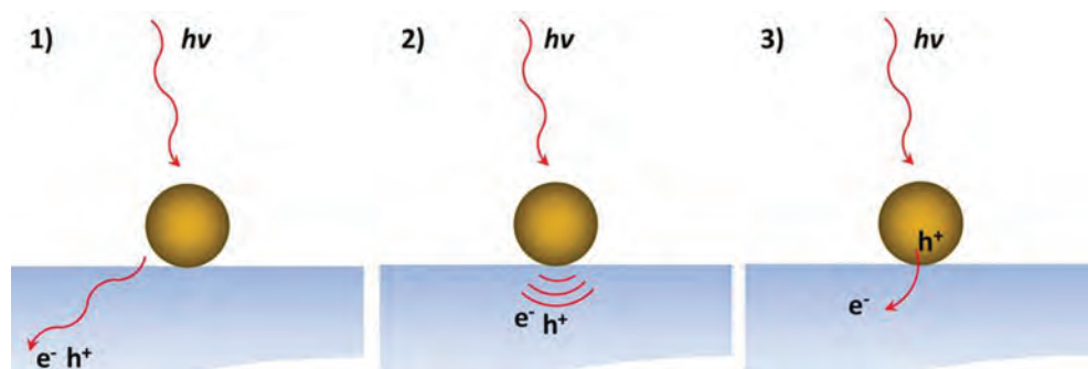
Figure 8. Schematic of different interactions between a metal nanoparticle and a photoactive substrate: (1) far-field scattering, (2) near-field scattering and (3) direct injection of photoexcited carriers into the semiconductor.
