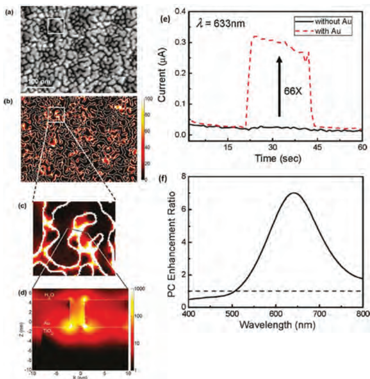
Figure 11. On the left, (a) SEM image of a 5-nm thick Au island film on TiO 2 ; FDTD-simulated electric field intensity, in the plane xy (b, c) and in a vertical section (d). On the right, (e) photocurrent of anodic TiO 2 with and without Au nanoparticles irradiated with \lambda = 633 nm light for 22 s; (f) photocurrent enhancement ratio spectrum; the dashed line refers to the bare TiO 2 (value 1). Reprinted with permission from Liu et al. [43]. Copyright ©2011, American Chemical Society.
