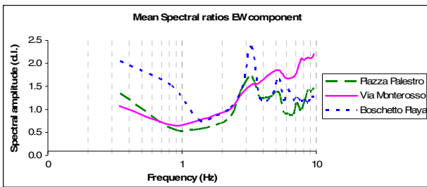
Figure 1. Mean spectral ratios calculated for the EW component of microtremor measurements for all stations used in the three sites in Catania.
