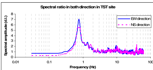
Figure 2. HV spectral ratios of the TST site.
