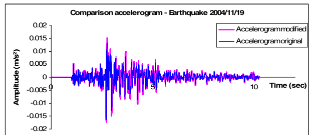
Figure 6. Comparison between original and modified accelerograms at the bedrock for the earthquake November 19 th 2004.
