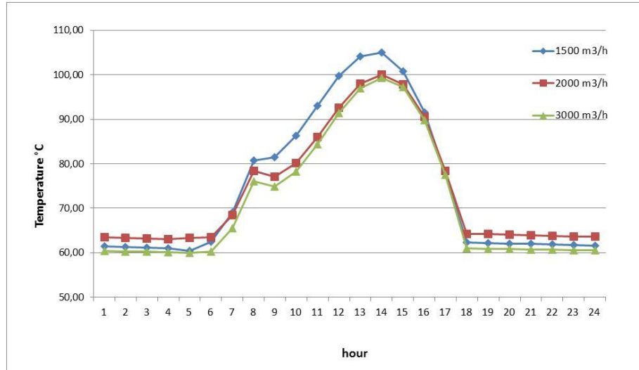
Figure 5. Thermal Storage temperatures
