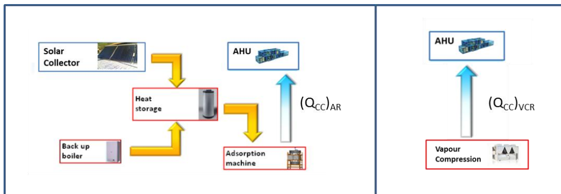
Figure 8. a) ARs configuration; b) VCRs configuration
