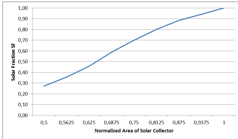
Figure 6. SF vs normalised Area of solar collector
