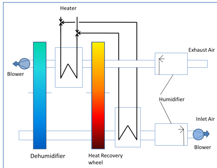
Figure 1. Scheme of Desiccant Cooling Systems
