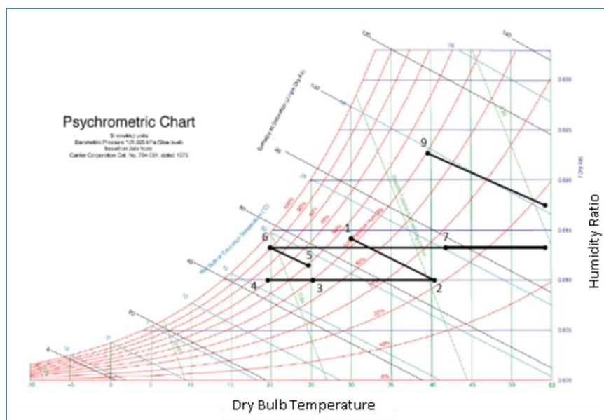
Figure 3. Thermodynamic transformations.
