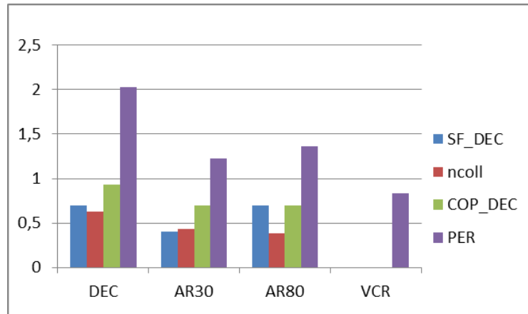
Figure 9. Comparison of energy performance indices
