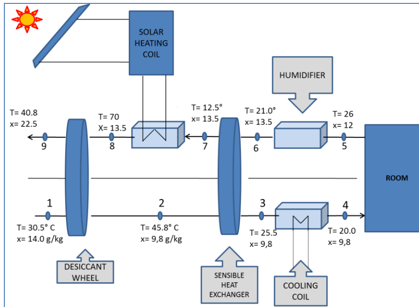
Figure 2. DEC system configuration
