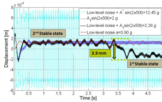
Fig. 2. Simulation results: in presence of noise level or sinusoidal bias of 0.9g (red) and 2g (blue) respectively, the system oscillates in a single-well (second stable state). The mixing of both allows switching between the two states (black). The last evolution represents the over-excited condition ( A^* \gg A_1 , cyan)
