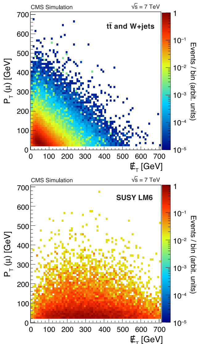
Fig. 1 Distributions of muon p_T vs. \cancel{E}_T in the \mu channel for simulated t\bar{t} and W + jets events (top) and for the LM6 SUSY benchmark model (bottom)
