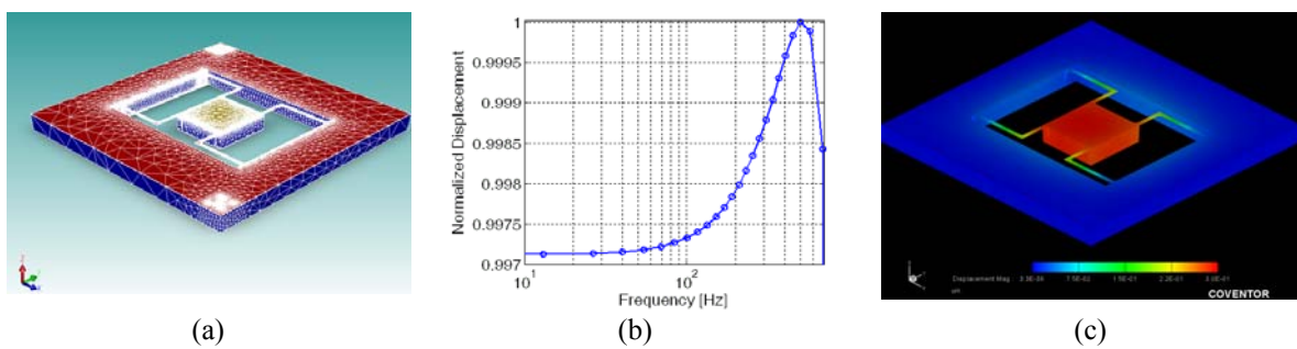
Fig. 3. (a) Tetrahedrons-based model mesh, (b) harmonic response along the z axis (normalized to its maximum value), (c) displacement color map in absence of applied load to the plate surface of the microresonator.
