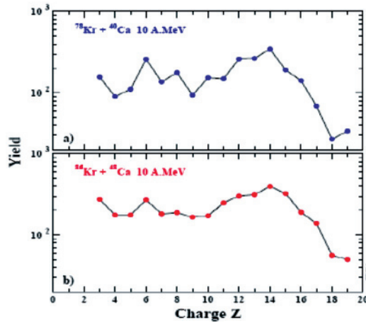
Figure 3: Charge yield of IMF for the n-poor system and the n-rich one, \theta = 10^\circ\text{-}13^\circ .
