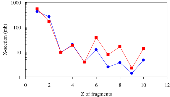
Figure 4: (Color Online) DNS calculation for fragments with atomic number Z such that 1 \leq Z \leq 10 . The red squares refer to the n-poor system (reaction ^{78}\text{Kr}+^{40}\text{Ca} ), whereas the blue circles refer to the n-rich one (reaction ^{82}\text{Kr}+^{40}\text{Ca} ).
