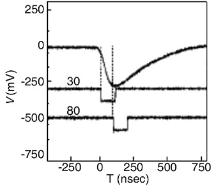
Figure 1: Signal rise-time as deduced by time difference between CFD's output at 30% and 80% of original signal.
