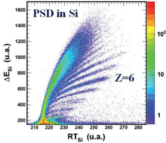
Figure 2: E-RiseTime plot for ^{78}\text{Kr}+^{40}\text{Ca} , at \theta = 34^\circ .
