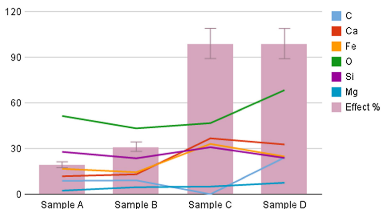
Figure 2 Profiles of the elements for which student's t test with Bonferroni's correction provided significant differences and toxic effect (0-100%) of the dust suspensions in relation to their per cent content in the elements found more frequently. Elements and % effect are distinguished by color as specified in the figure.
