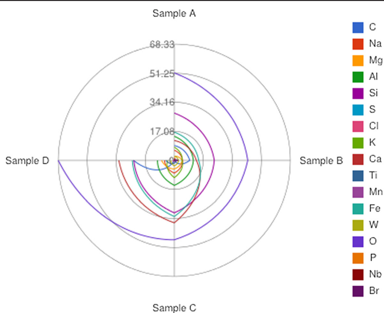
Figure 1 Concentrations of the elements found more frequently in the four samples (% weight). Elements are distinguished by color as specified in the figure.
