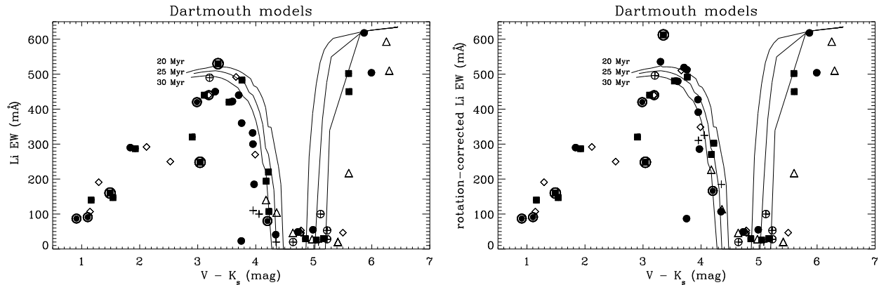
Fig. 5. Left panel: distribution of Li EWs versus V - K_s color for \beta Pic members. Solid lines represent the Li EWs predicted by the Dartmouth models for ages in the range from 20 to 30 Myr. Right panel: same as in the left panel, but Li EW decoupled from rotation, assuming that fast rotators have rotation-affected Li EW.
