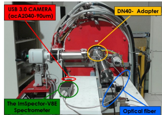
Figure 2. A view of the FPT and the OES set-up.
