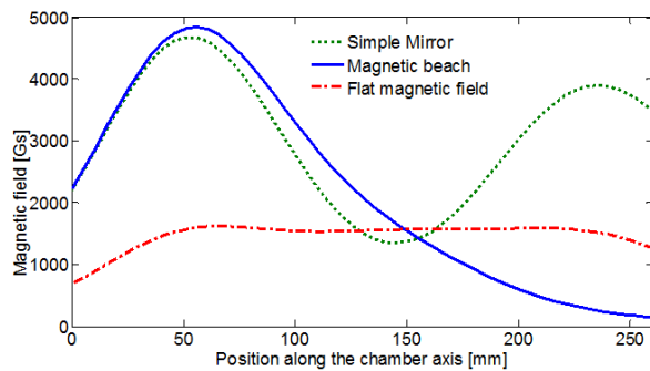
Figure 1. Magnetic field profiles that can be generated by the FPT.
