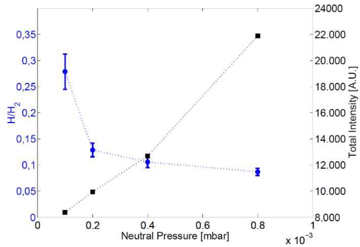
Figure 4. Dependence of the n_H/n_{H_2} ratio on the pressure.
