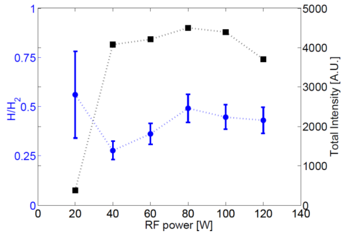
Figure 3. Dependence of the n_H/n_{H_2} ratio on RF power.
