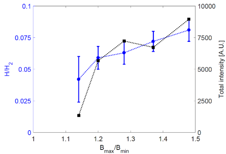
Figure 5. Dependence of the n_H/n_{H_2} ratio on the B_{max}/B_{min} ratio.
