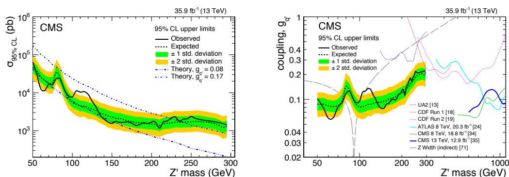
Figure 7. The 95% CL upper limits on the Z^0 boson production cross section compared to theoretical cross sections (left) and on the quark coupling g_{q^0} as a function of resonance mass for a leptophobic Z^0 resonance that only couples to quarks (right). The observed limits (solid), expected limits (dashed) and their variation at the 1 and 2 standard deviation levels (shaded bands) are shown. Limits from other relevant searches and an indirect constraint on a potential Z^0 signal from the SM Z boson width [72] are also shown.
