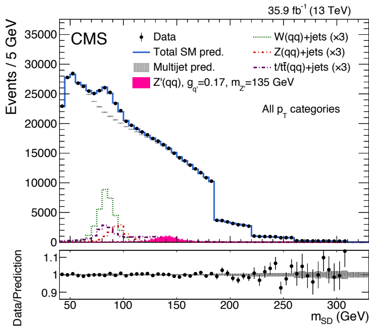
Figure 10. Soft-drop jet mass distribution for the passing region and combined p_T categories. The multijet background prediction in the passing region is obtained using the failing region and the pass-fail ratio R_{p=f}(m_{SD}, p_T) . Data are shown as black points. The multijet background prediction, including uncertainties, is shown by the shaded bands. Contributions from the W and Z boson, and top quark background processes are shown, scaled up by a factor of 3 for clarity. A hypothetical Z^0 boson signal at a mass of 135 GeV is also indicated. The features at 45, 185, 220 and 255 GeV in the m_{SD} distribution are due to the kinematic selection on \rho , which affects each p_T category differently. In the bottom panel, the ratio of the data to the background prediction, including uncertainties, is shown.
