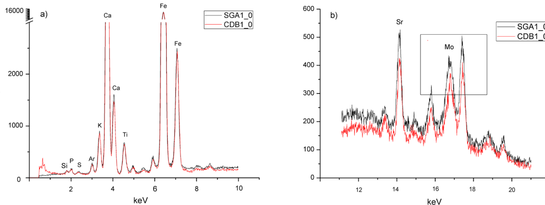
Figure 4. Comparison between the X-ray Fluorescence spectra of selected clays, not purified nor sieved: SGA1_0 and CDB1_0, in the energy regions 1-10 keV (a) and 10-20 keV (b). The three peaks in the high energy region come, in order of decreasing energy, from Rayleigh diffusion, Compton scattering and escape peak of anode Mo.
