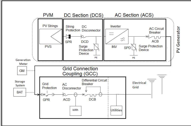
Fig. 3. Schematic decomposition of the PV system
