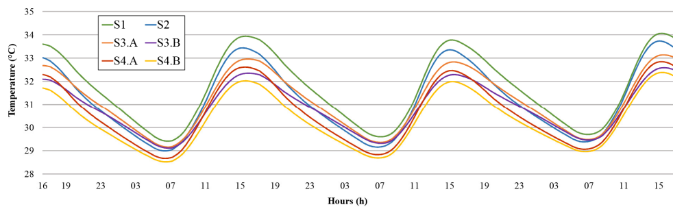
Figure 5. Indoor air temperature of the proposed scenarios
