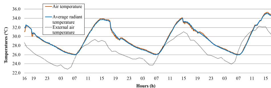
Figure 3. Temperature measured during the monitored period
