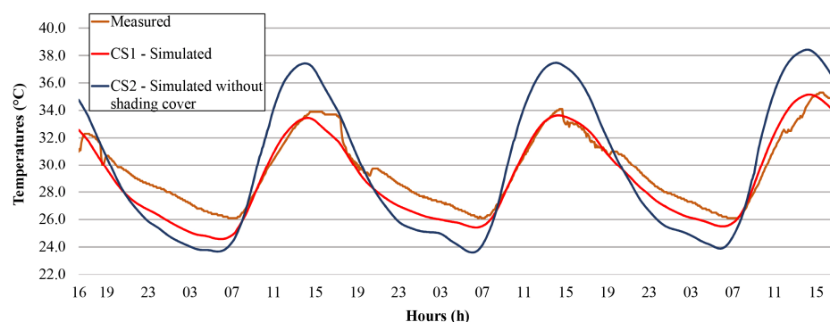
Figure 4. Energy Plus model validation – measured vs. simulated air temperature
