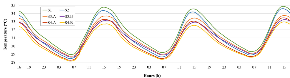
Figure 7. Inside surface temperature of the proposed scenarios
