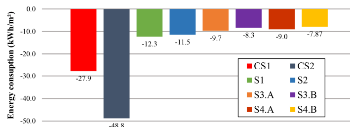
Figure 8. Energy needs for space cooling
