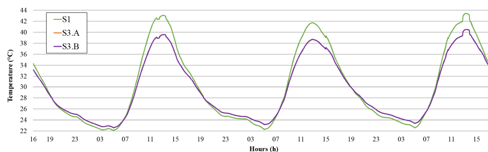
Figure 6. Outside surface temperature of the proposed scenarios
