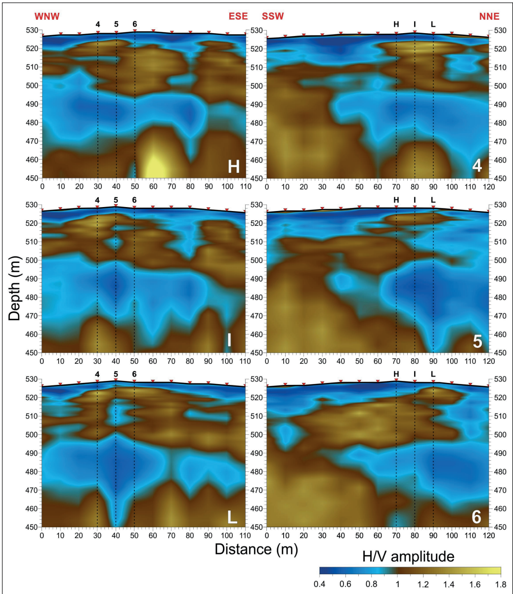
Fig. 3 - Impedance contrast sections obtained from seismic ambient noise samplings (see Fig. 1d for location).
