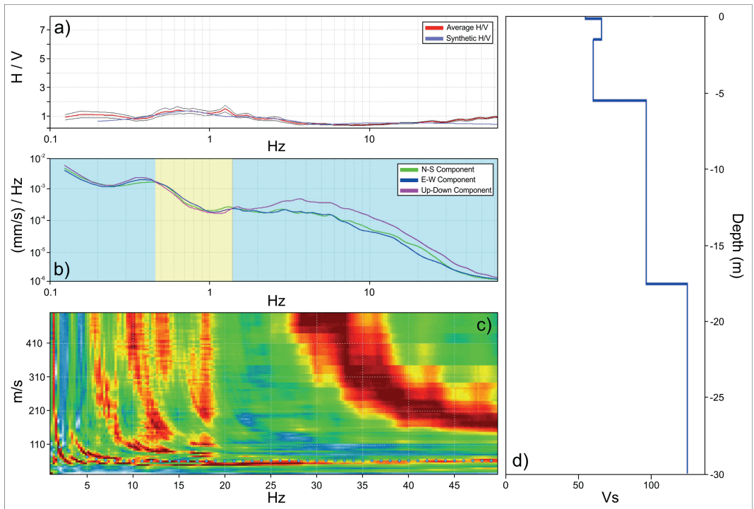
Fig. 2 Joint fit between HVSR spectrum (a), relating to one seismic ambient noise record (G6) acquired near the MASW survey (see fig. 1d for location) and Rayleigh waves dispersion curve (c), obtained from the MASW survey; b) example of single component spectra, related to one seismic ambient noise sampling (G6) (the area highlighted in yellow show the typical eye-shape, the two blue area highlight the possible presence of areas characterized by velocity inversion) d) velocity-depth profile obtained from MASW-HVSR joint fit.
