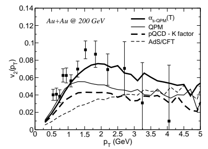
Figure 3. v_2 as a function of p_T for the minimum bias Au+Au collisions.
