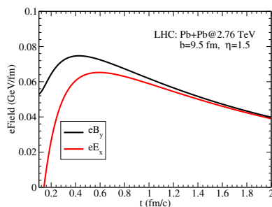
Figure 4. Time evolution of the magnetic field eB_y and the electric field eE_x in the forward rapidity region.
