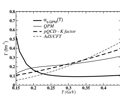
Figure 1. Drag coefficients as a function of temperature.
