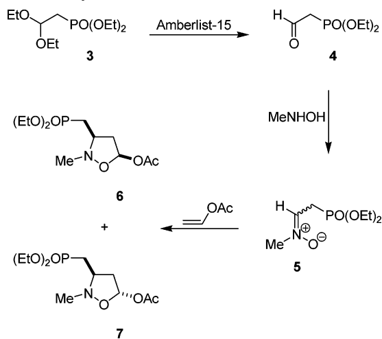
Figure 1. Carbocyclic 2'-oxa-3'-aza-nucleosides.
