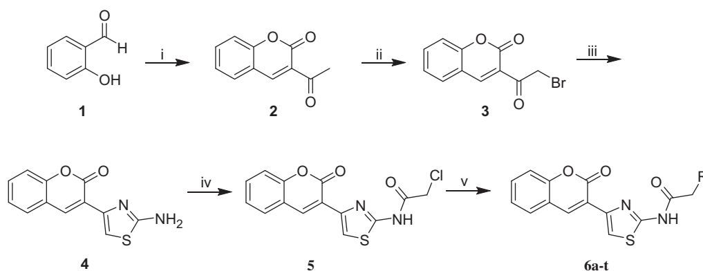
Scheme 1. Synthesis of new coumarylthiazole-substituted acetamide derivatives. Reaction conditions: (i) Ethylacetoacetate, piperidin, rt, 30 min; (ii) Br 2 , CHCl 3 , 50 °C, 15 min; (iii) Thiourea, EtOH, 80 °C, 2 h; (iv) Chloroacetylchloride, Et 3 N, THF, 70 °C, 8 h; (v) RNH 2 , DMF, 60 °C, 12 h.
