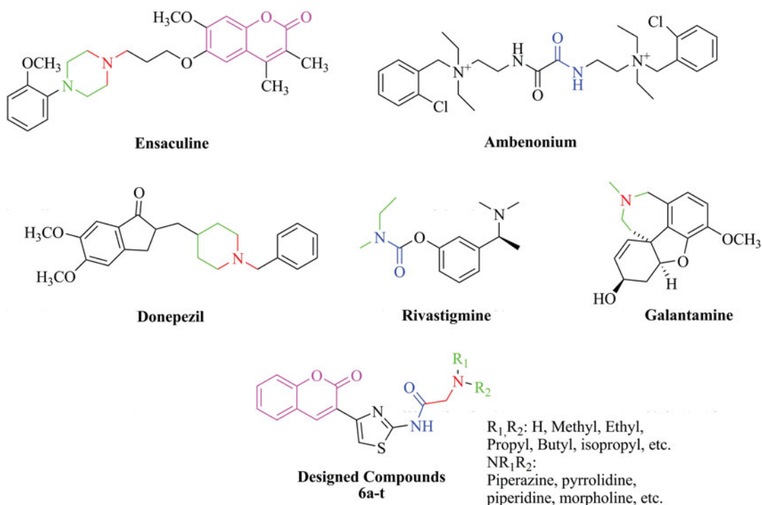
Figure 1. Structures of well-known cholinesterase inhibitors and designed compounds.
