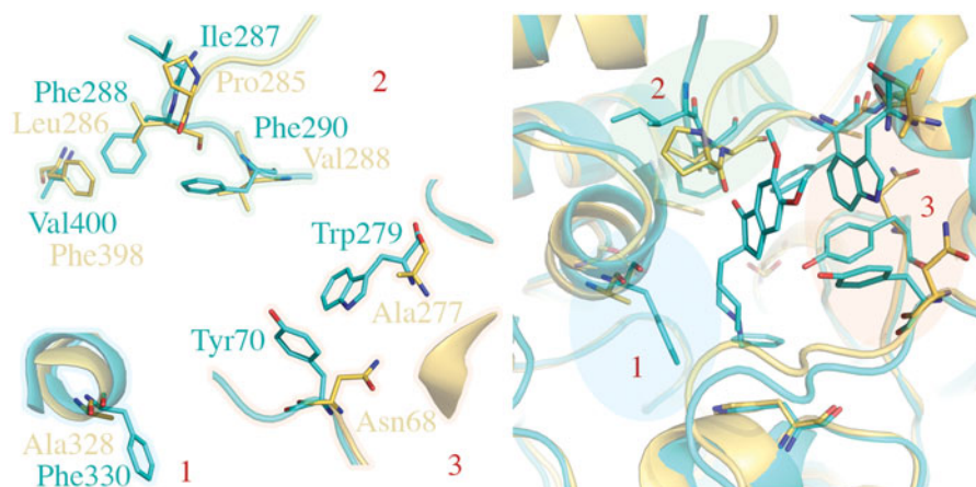
Figure 5. Comparison of TcAChE (1EVE residue Ile287, Phe288, Phe290, Val400, Trp279, Tyr70, Phe330, in blue) and hBuChE (1P0M residue Pro285, Leu286, Val288, Phe398, Ala277, Asn68, Ala328, in gold). The most important changes in aminoacids sequence are highlighted by blue, green and red areas. As shown, modifications generally affect both CAS (1, in blue) and PAS (2, in green and 3, in red).
