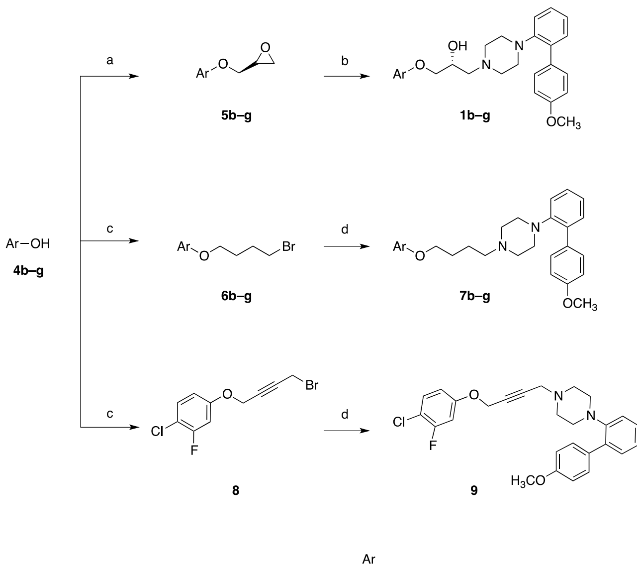
Scheme 1. a
