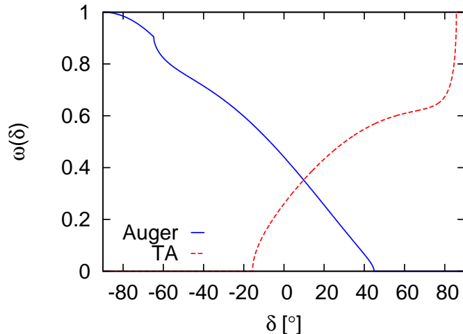
Figure 4. The geometrical relative exposures of the Pierre Auger Observatory and Telescope Array as a function of declination. Both distributions have been normalized to unity at the declinations where the exposure is maximum for each experiment. To simulate signal events, the decision whether each event is a cosmic ray measured by Auger or by TA is done with a probability given by the fraction of the number of events measured by each Observatory.
