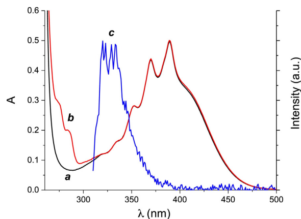
Fig. 6. Absorption spectra of an aqueous solution of AN- \beta CD-NOPD ( 30 \mu\text{M} ) (a) and its complex with naphthalene (b) (left Y-axis). Fluorescence emission spectrum (c) observed upon excitation at \lambda_{\text{exc}} = 280 nm of the sample b (right Y-axis).
