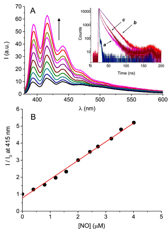
Fig. 4. (A) Fluorescence ( \lambda_{\text{exc}} = 370 nm) spectral changes observed upon irradiation of an aqueous solution of AN- \beta CD-NOPD ( 40 \mu\text{M} ) at regular irradiation times of 5 min (from bottom to top) with visible light ( \lambda_{\text{exc}} = 405 nm). The inset shows the fluorescence decay and the related multiexponential fitting for solutions of AN- \beta CD-NOPD (a), the model compound AN- \beta CD (b) and AN- \beta CD-NOPD after 45 min irradiation with visible light (c); \lambda_{\text{exc}} = 370 nm; \lambda_{\text{em}} = 420 nm. (B) Correlation of the fluorescence increase observed in Fig. 4A and the concentration of NO released from the same solution ( I and I_0 represent the fluorescence intensities at 420 nm after each irradiation time and that of the non-irradiated solution, respectively).
