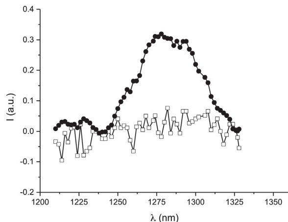
Fig. 5. Luminescence spectra detected upon 370 nm light excitation of a \text{D}_2\text{O} solutions of AN- \beta CD-NOPD ( 40 \mu\text{M} ) before ( \square ) and after ( \bullet ) 1 h irradiation at \lambda_{\text{exc}} = 405 nm.
