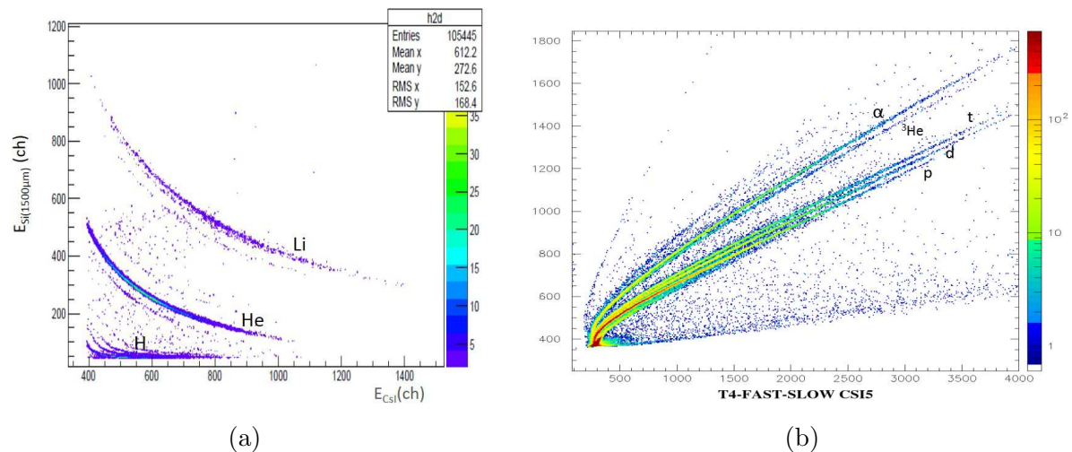
Figure 5. Preliminary spectra from INKIissy experiment data related with FARCOS demonstrator. (a) E- \Delta E spectrum combining 1500 \mu\text{m} DSSSD ( \Delta E ) and CsI(Tl) (E) signals. (b) Fast-Slow spectrum coming from the particles detected by CsI(Tl) crystals. Both spectra show the excellent resolution of a FARCOS telescope for mass and charge separation.
