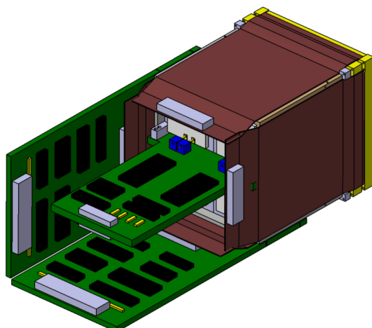
Figure 7. Rear view of the new design for a FARCOS telescope. Four dedicated ASIC boards will be mounted to the telescope (two are shown in the drawing), to manage the signals and bias voltages from DSSSD's, to which are connected by means of kapton cables. In the rear-middle, a single circuit will manage voltages and signals for four CsI(Tl) crystals.
