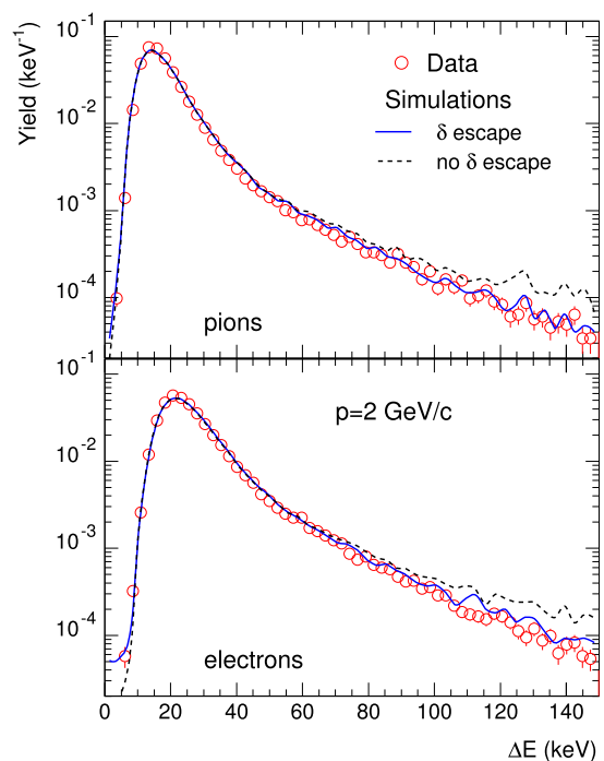
Fig. 6. Distributions of the ionisation energy loss of pions and electrons with momenta of 2 \text{ GeV}/c . The symbols represent the measurements obtained at the CERN PS with prototype read-out chambers that were smaller in overall size (active area 25 \text{ cm} \times 32 \text{ cm} ) but otherwise similar in construction to that of the final detector. The lines are simulations accounting (continuous line) or not (dashed line) for the long range of \delta -electrons as compared to the chamber dimensions. Figure taken from [48].
