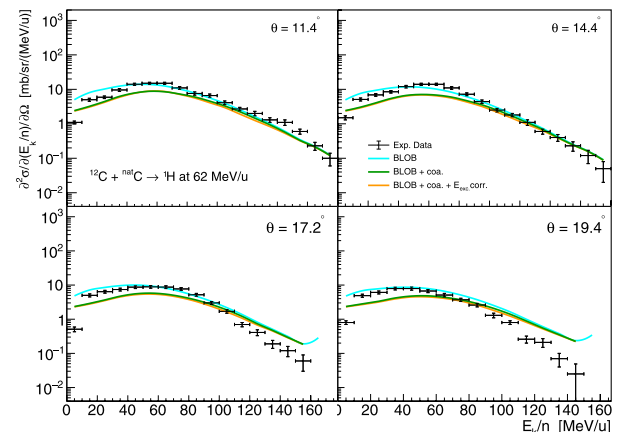
Fig. 11. Same as Fig. 10 but for protons.
