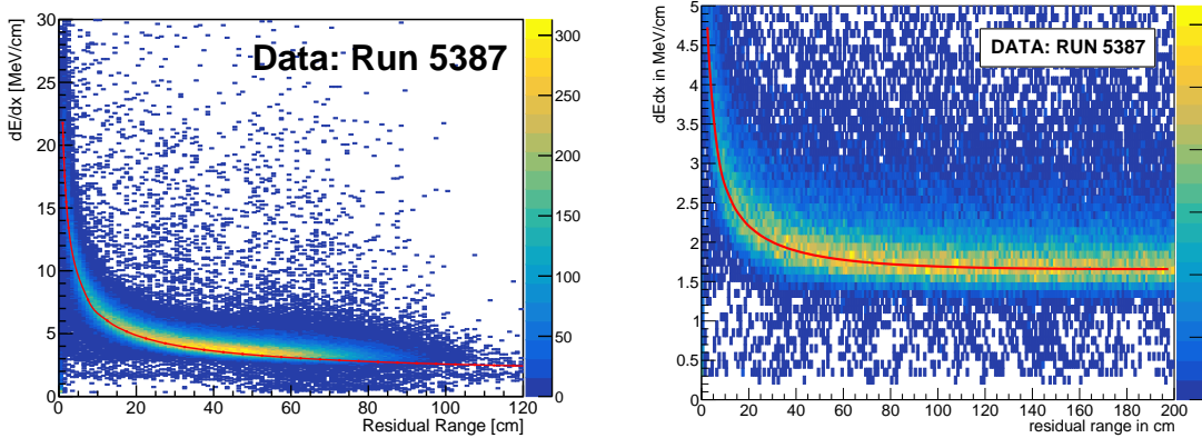
Figure 2.13. Energy loss of protons (left) and muons (right) in 1-GeV running with the ProtoDUNE-SP LArTPC at CERN, as a function of residual range. The protons are beam particles identified from beamline instrumentation; the muons are reconstructed stopping cosmic rays collected concurrently. The red curves represent the mean of the corresponding expected signature. Note the difference in the vertical scale of the two plots. The kaon dE/dx curve will lie between the two curves shown.
