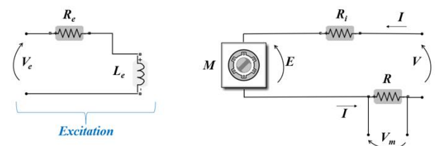
Figure 1. Equivalent circuit of the drill.
