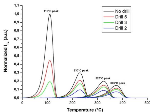
Figure 3. Comparison among the simulated normalised glow curves obtained for the different sampling conditions. The No Drill condition is obtained by the deconvolution of an experimental glow curve of an original terracotta sample.
