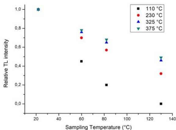
Figure 2. Intensity trend vs drilling temperature for all TL peaks.
