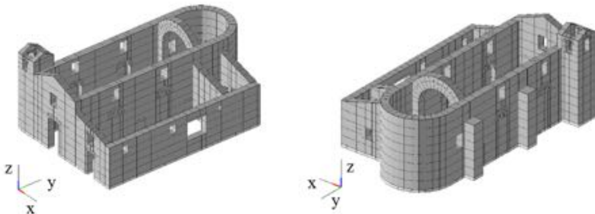
Figure 8: Numerical model and adopted reference system.
