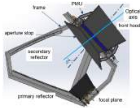
Fig. 12. LFT structure.
