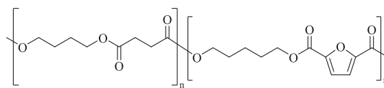
Fig. 1. General chemical structure of P(BS- b -PeF) x copolymers.
