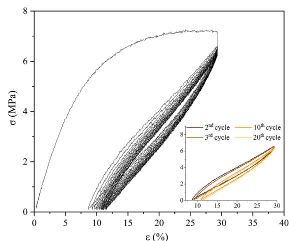
Fig. 8. Stress–strain curve obtained from the cyclic test of the sample P(BS- b -PeF) 3 at 30% of maximum elongation. Insert: 2nd, 3rd, 10th and 20th cycles.
