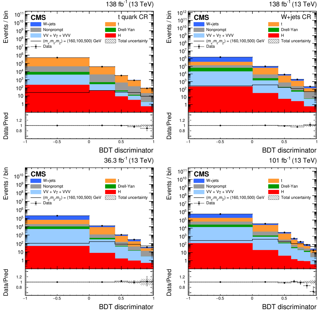
Figure 4. Post-fit BDT distributions in the \ell\nu qq channel for the full data set in the t quark CR (upper left) and W +jets CR (upper right). The SR of the 2016 data set (lower left) and the 2017–2018 data set (lower right). The black line indicates the signal prediction with m_s = 160 GeV, m_\chi = 100 GeV, m_{Z'} = 500 GeV. In the lower panel of each plot, the ratio between the data and the background prediction is shown.
