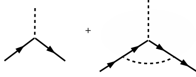
Figure 1.18: Diagrammatic representation of the 1PI \Gamma_{\psi\bar{\psi}\sigma}^b , calculated in Eq. (1.169) by means of the perturbative expansion in the bosonized version of the model.
