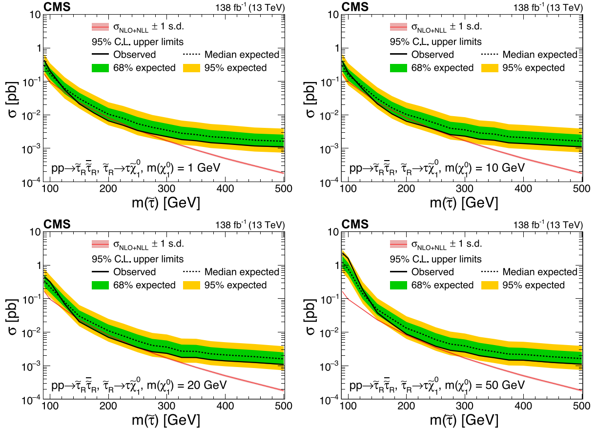
FIG. 6. Expected and observed 95% CL cross section upper limits as functions of the \tau mass in the purely right-handed \tau scenario for \chi_1^0 masses of 1, 10, 20, and 50 GeV (upper left to lower right). The inner (green) band and the outer (yellow) band indicate the regions containing 68% and 95%, respectively, of the distribution of limits expected under the background-only hypothesis. The red line and thin shaded band indicate the NLO + NLL prediction for the signal production cross section calculated with RESUMMINO [30], and its uncertainty.
