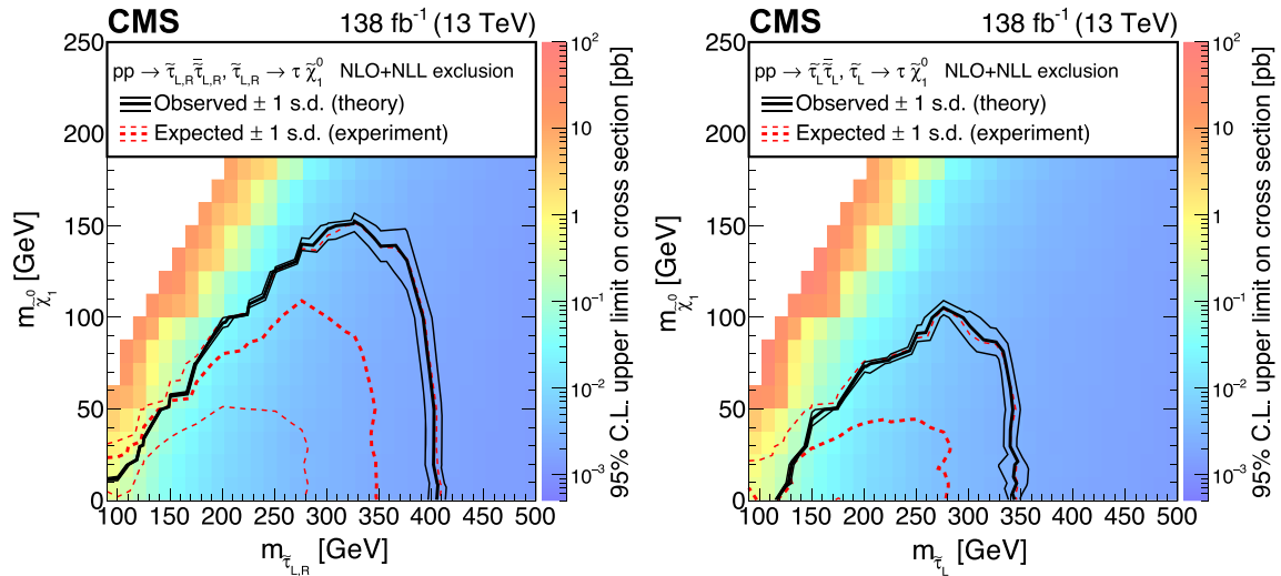
FIG. 7. Upper limits at 95% CL on the cross section for degenerate (left) and purely left-handed (right) \tau pair production in the m(\tau) - m(\chi_1^0) plane. The thick black (red) curves show the observed (expected) exclusion limits assuming NLO + NLL predictions for the signal cross sections. The thin black curves represent the variations in the observed limits obtained when these cross sections are varied by their \pm 1 standard deviation uncertainties. The thin dashed red curves indicate the region containing 68% of the distribution of limits expected under the background-only hypothesis.
